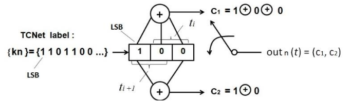
Figure 3. Example of a MM with the input sequence \{k_n\} generating an output sequence out_n(t) = (c_1, c_2) .
