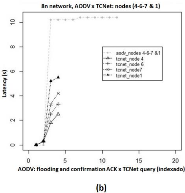
Figure 8. (a) Comparison of 1 TCNet query and AODV signaling mechanism to establish a route to node 4; (b) Scenario of comparing TCNet queries for an 8-node network with respect to AODV.
