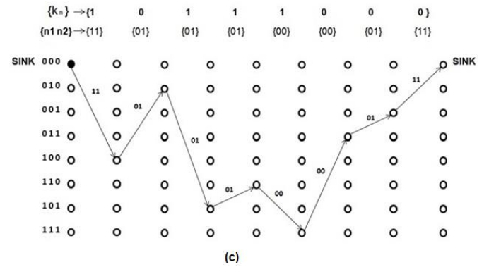
Figure 7. (a) Mealy machine (MM) with k/n=1/2 , resulting output words (n_1, n_2) ; (b) Trellis diagram corresponding to MM; (c) Theoretical result of the route over the trellis due to a query.
