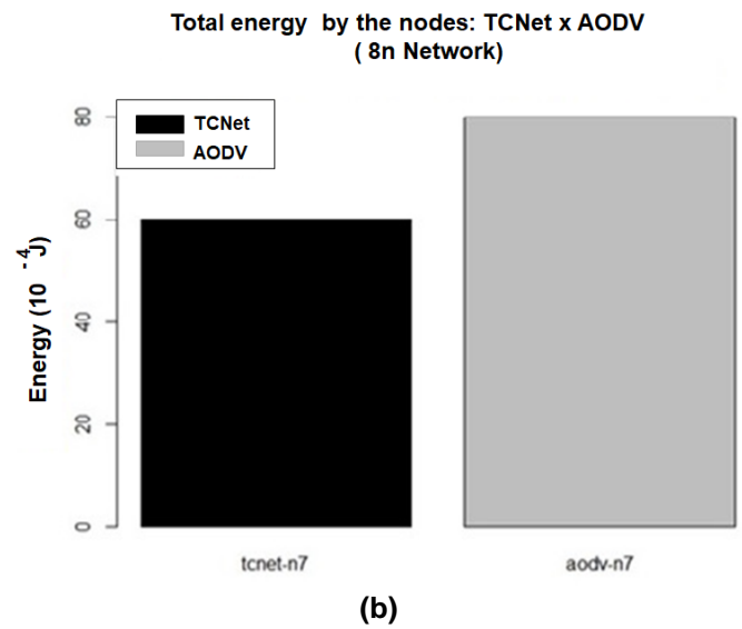
Figure 9. (a) Energy distributed among TCNet nodes in relation to the energy consumed by the AODV; (b) Comparison between the total energy consumed by the mechanisms of TCNet x AODV.
