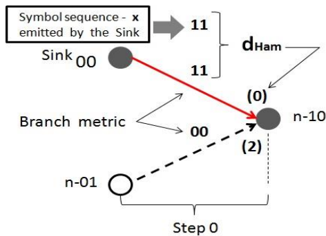
Figure 5. Example of hard decision used by state ( n - 10 ) to decide on a trellis branch, based on received sequence {11}.
