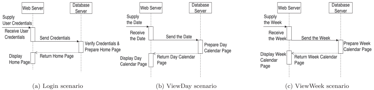
Figure 2: Message sequence charts of WebCalendar requests (scenarios)
