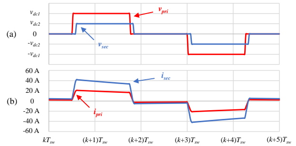
Figure 12. Waveforms in the primary and secondary sides of the HF transformer when the DAB operates under DPS modulation: (a) Voltage; (b) Current.
