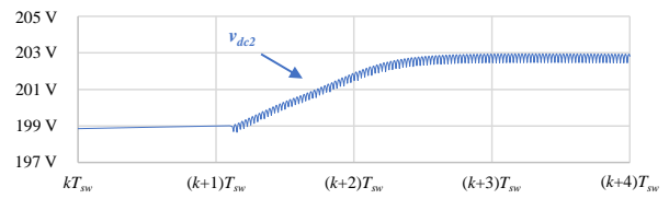
Figure 16. Secondary dc-link voltage ( v_{dc2} ) regulation considering an EPS modulation.
