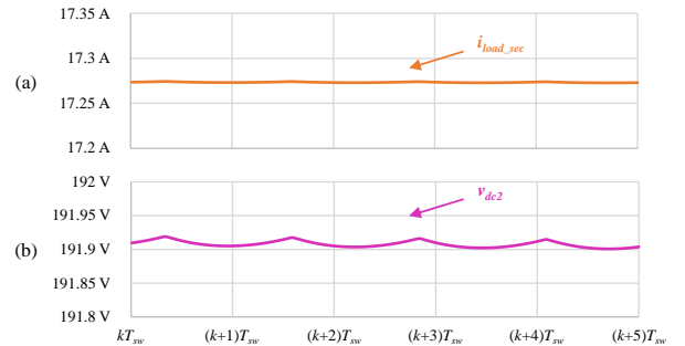
Figure 4. Waveforms in the secondary side resistive load when the SAB operates under Duty-Cycle Modulation: (a) Current; (b) Voltage.
