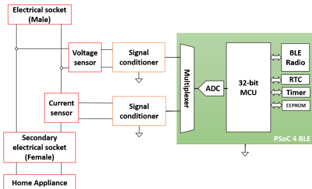
Figure 5. Monitoring device block diagram.
