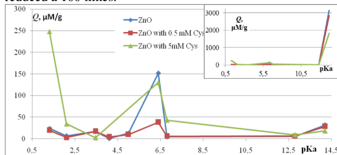
Figure 3. Distribution curves of acid-base sites on the ZnO nanostructures surface obtained at different Cys concentrations (on the insert are shown distribution curves without scaling peaks)
