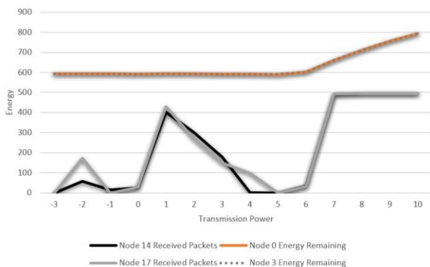
Figure 12. Remaining Energy and Packets Sent/Received vs Transmission Power under Scenario 2a.
