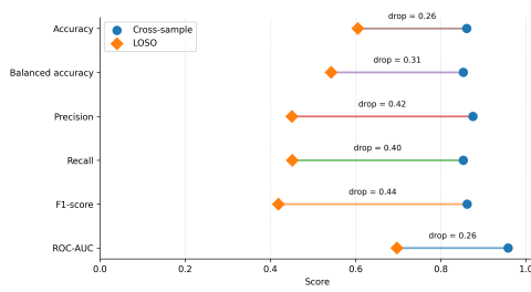
(a) Cross-sample vs. LOSO performance
