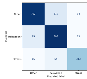
(b) Cross-sample confusion matrix
