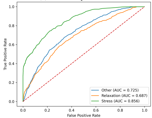
(b) LOLO ROC curves
