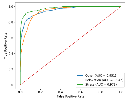
(a) Cross-sample ROC curves
