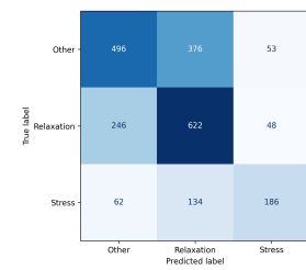
(c) LOSO confusion matrix
