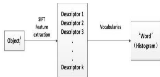
Figure 6. The process about creating a 'word' for one sample image in the train set.
