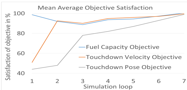
Figure 10: Our approach successfully changes the vehicle configuration in order to increase the simulation goal satisfaction.
