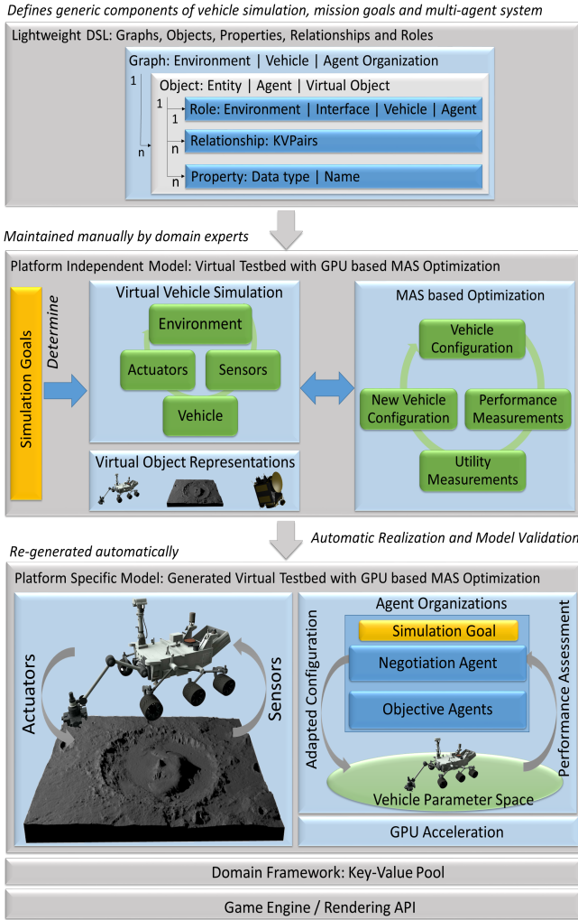
Figure 2: Overview of our proposed approach. From a lightweight DSL, graphical Platform Independent Models (PIM) are modelled which are used to generate our virtual testbed with its vehicle simulation and configuration optimization.
