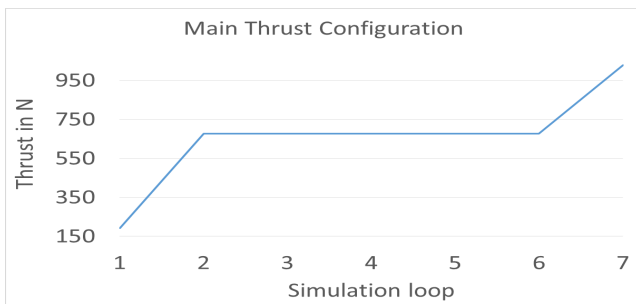
Figure 11: Our approach gradually increases the thrust level until the velocity can be adequately regulated for landing.
