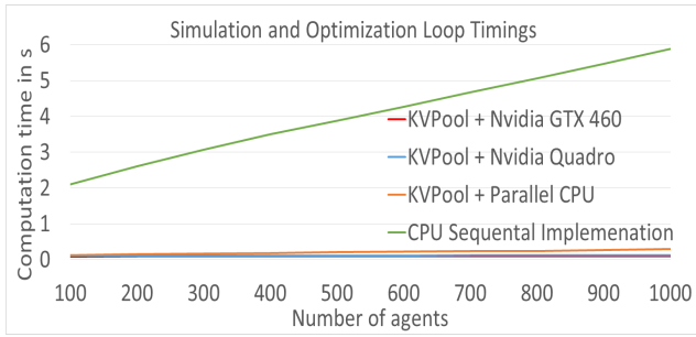
Figure 8: Computation time for one simulation and optimization run.
