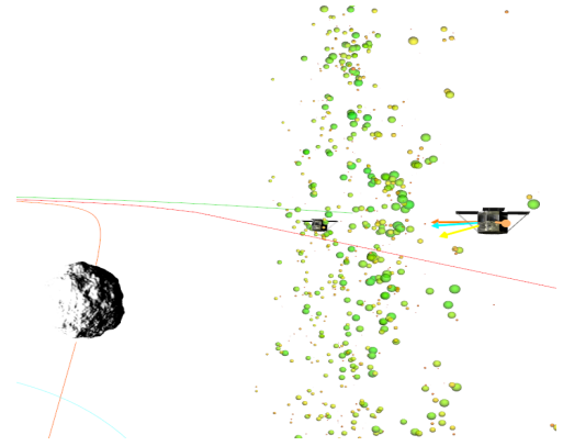
Figure 7: Example rendering of our approach within KaNaRiA [22]: On-board particle filter localization (color-coded spheres) before landing of our simulated spacecraft.
