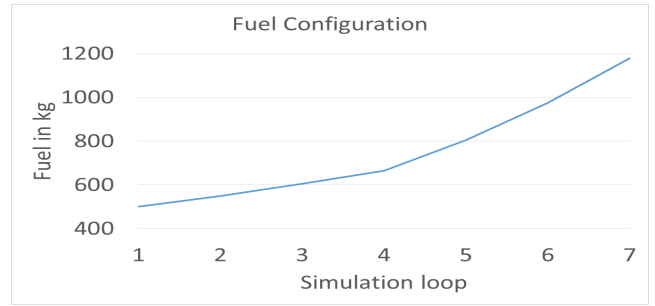
Figure 12: Our approach gradually increases the fuel capacity in order to maintain thrust while the landing procedure is conducted.
