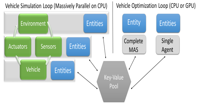
Figure 3: Entities are mapped to our generic vehicle simulation loop, consisting of the environment, sensors, actuators and internal vehicle components. Our MAS is either computed on the CPU with n Entities or on the GPU as one Entity with a single CUDA kernel for all agents.
