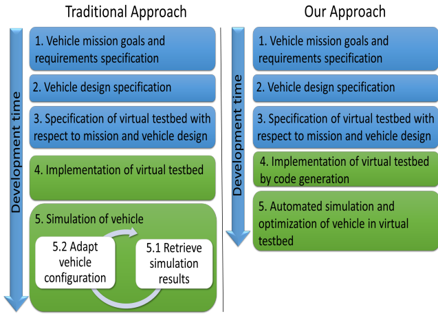
Figure 1: Integration of virtual testbeds with the vehicle engineering process: Simulation results are used to change vehicle configurations in order to meet engineer expectations if the simulated vehicle performance does not meet vehicle mission or engineering expectations. In the traditional approach, virtual testbed development as well as actual vehicle simulation take the most of the overall engineering process time (left). Our approach (right) reduces this development time significantly by introducing source code generation as well as autonomous vehicle optimization without supervision.
