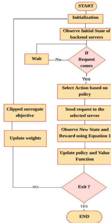
Figure 3: Proximal Policy Optimization Flowchart
