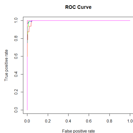
Figure 5. ROC Curve for Random Forest
