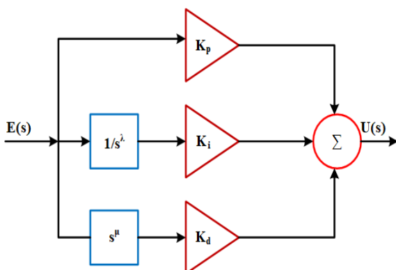
Figure 4. FOPID Controller
