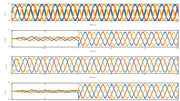
Figure 5. Analysis of V_s , I_s , I_L , I_c during starting condition
