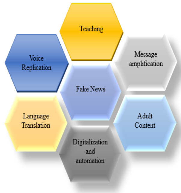
Figure 3. Deepfake applications
