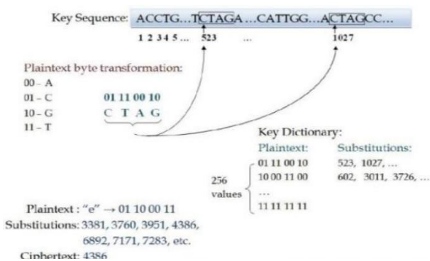
Figure 1. Encryption in DNA Indexing Algorithm
