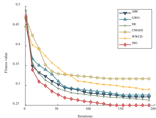
Figure 12. Results of the number of convergence iterations for each optimization network to improve the DBN network
