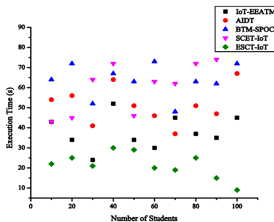
Figure 9. Execution Time
