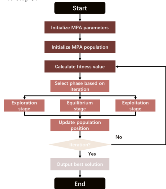
Figure 7. Flowchart of the marine predator algorithm
