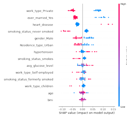
Figure 4. Model interpretability with SHAP summary plot
