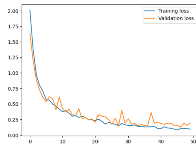
Figure 6. (b) Loss over Training and Validation
